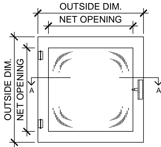
PLAN VIEW NOT TO SCALE
