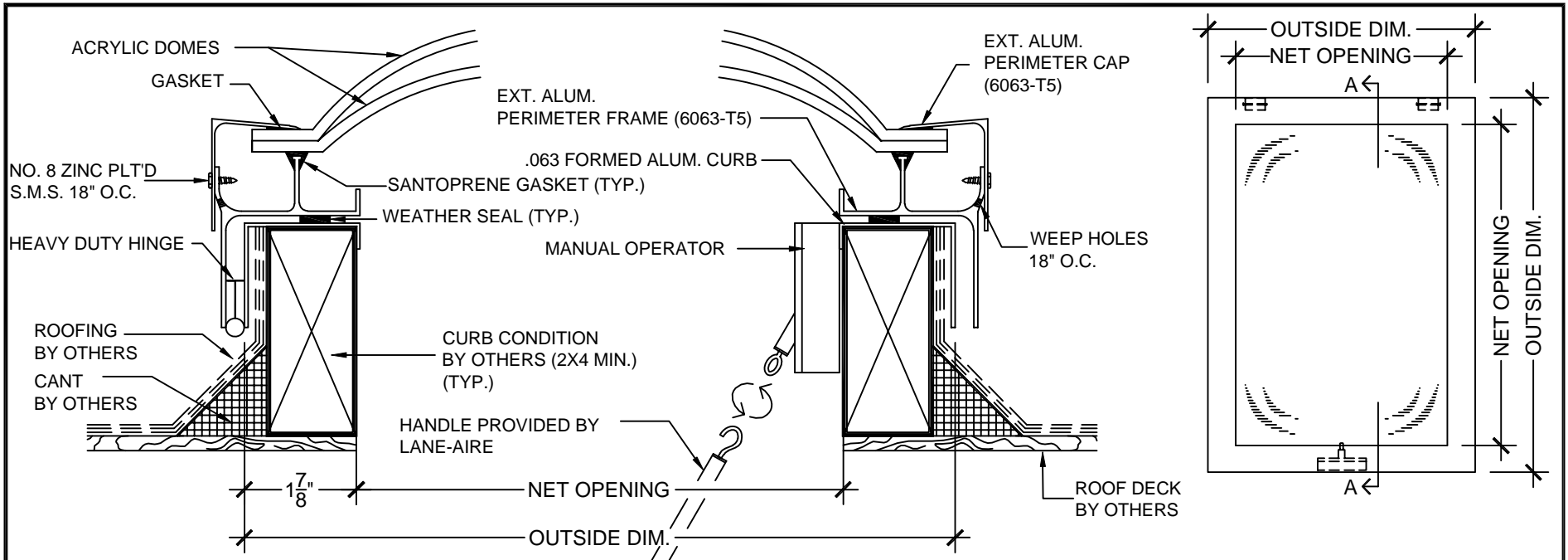
SECTION A - A SCALE : 3/8" = 1"
