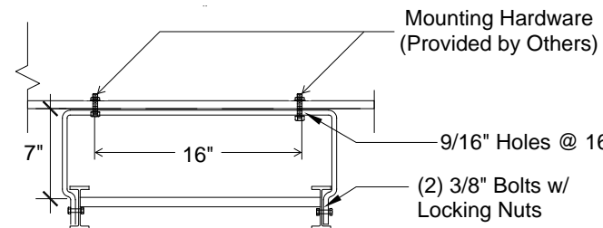
(C) Wall Bracket Plan View
